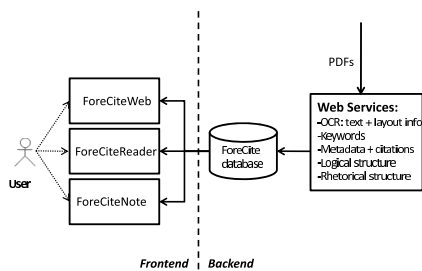
Figure 1: ForeCite architecture.
